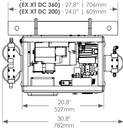
Compact Frame Top View
