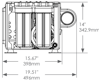
Compact Frame Side View
