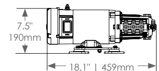
HP Pump (EX XT DC 360/600)
