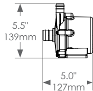
Booster Pump (48V)
