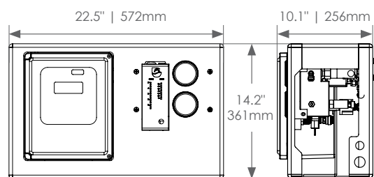
EPX1M – One Piece Modular
