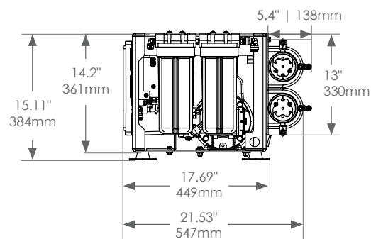
EPX1C – Compact Frame
