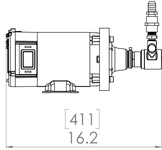
400 GPD - HP MOTOR PUMP ASSEMBLY
