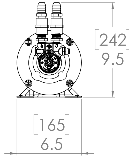
400 GPD - HP MOTOR PUMP ASSEMBLY
