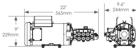
HP Pump
