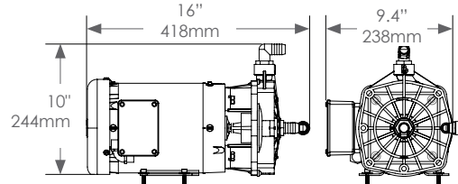
Booster Pump
