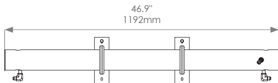
Vessel Assembly 400-1 / 600-1
