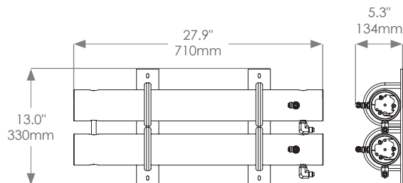
Vessel Assembly 400-2 / 600-2
