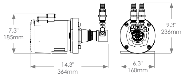
HP Motor Pump Assembly 400 GPD
