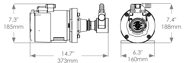
HP Motor Pump Assembly 600 GPD
